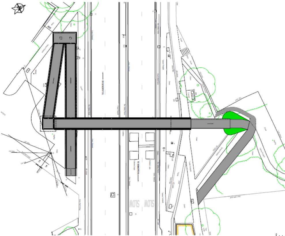
PLAN SCALE 1:150
