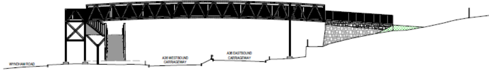
ELEVATION A SCALE 1:150
